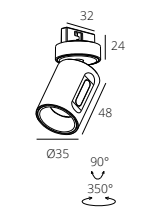
RCZ-MZ03/5W
